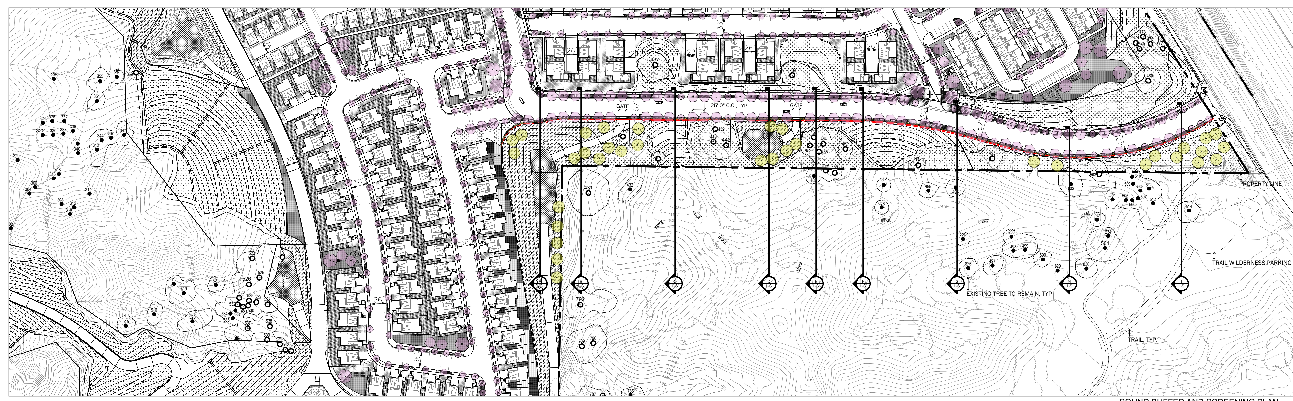
SOUND BUFFER AND SCREENING PLAN 1" = 100' - 0"
